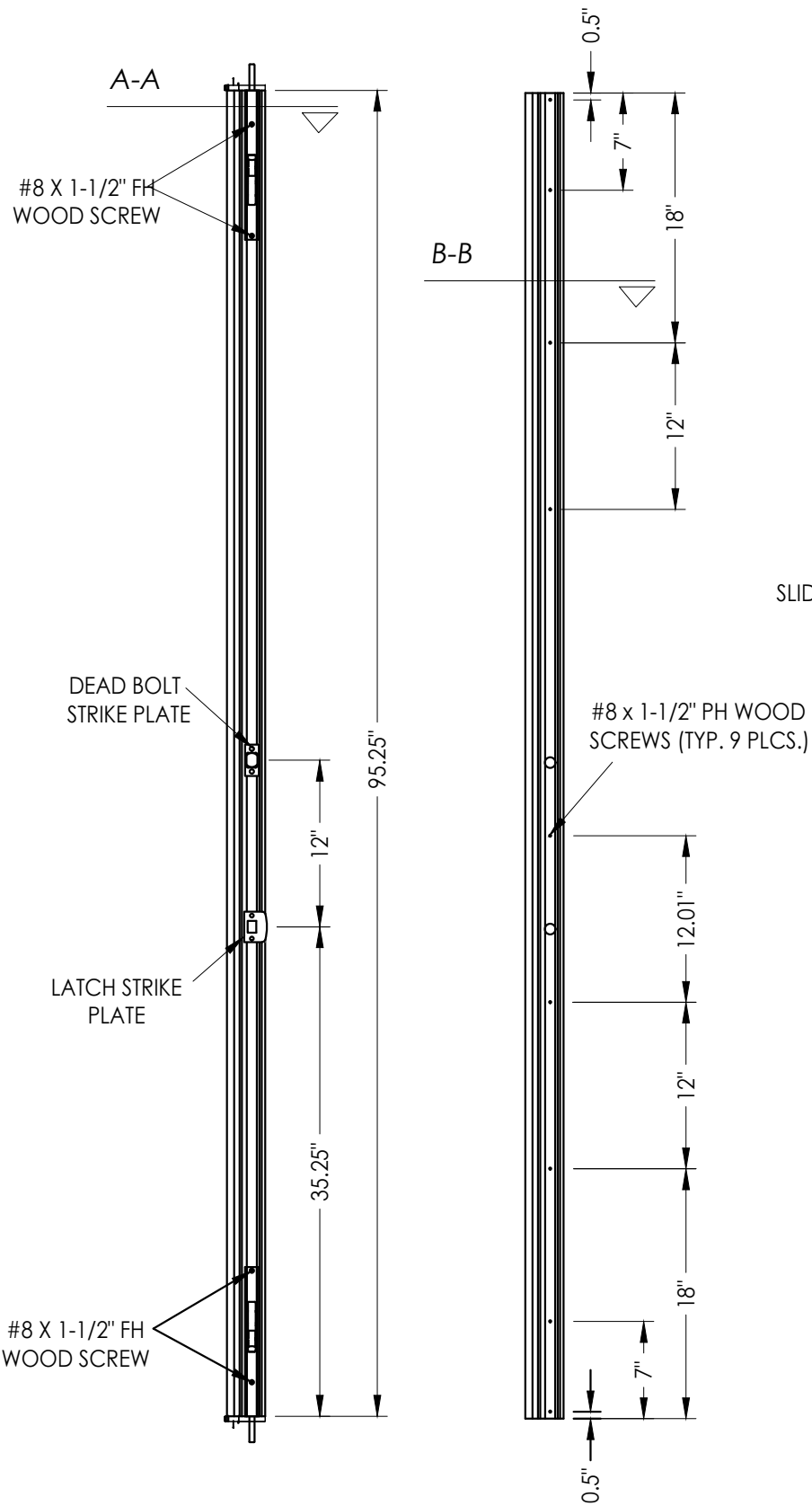
16 HURRICANE "T" ASTRAGAL by AFco Aluminum
