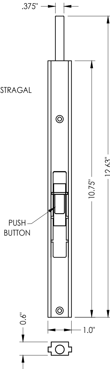
SLIDE BOLT ASSEMBLY (w/ Push Button) Aluminum
