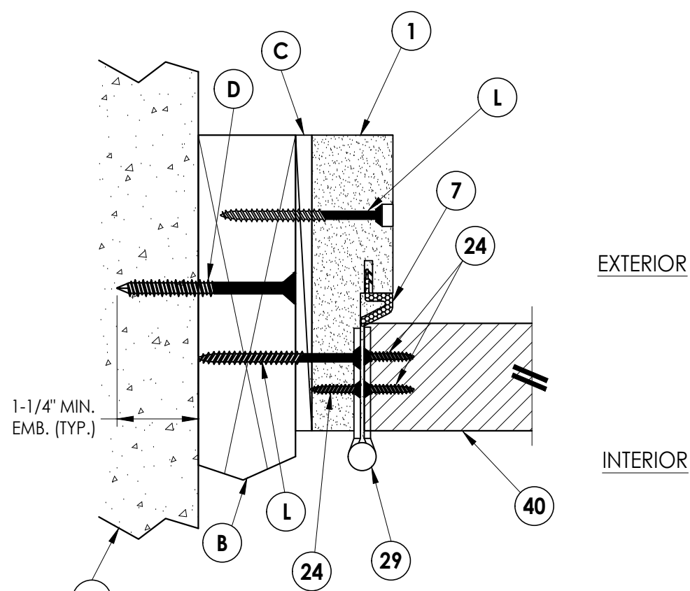
4 HORIZONTAL CROSS SECTION 3 Inswing shown Outswing also approved
