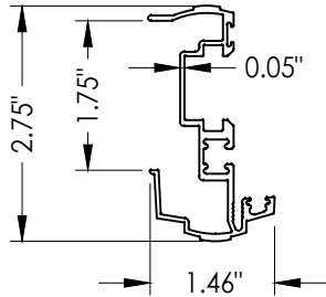
"T" ASTRAGAL PROFILE
