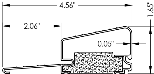
15 OUTSWING THRESHOLD AFCO H-497
