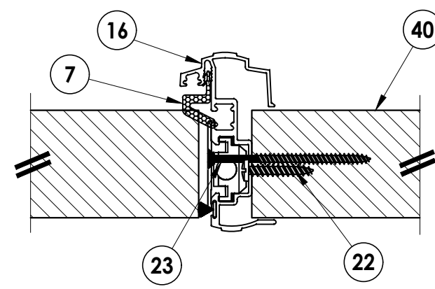
5 HORIZONTAL CROSS SECTION 3 Inswing shown Outswing also approved
