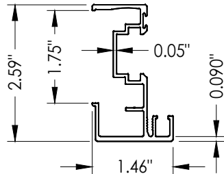
"T" ASTRAGAL FLAT PROFILE
