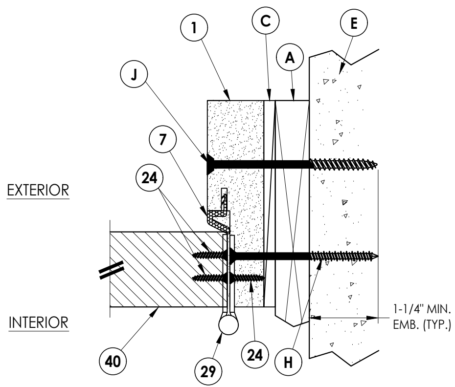
6 HORIZONTAL CROSS SECTION 3 Shown w/1X sub-buck
