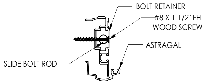
SECTION A-A Astragal Assembly
