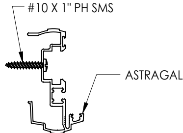
SECTION B-B Astragal Assembly
