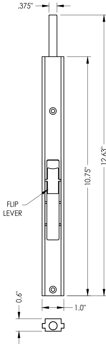
SLIDE BOLT ASSEMBLY (w/ Flip Lever) Aluminum
